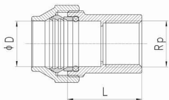
Racor recto hembra PE/H Female coupling PE/F
