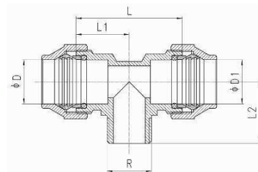
Racor "T" Macho PE/M Male Tee PE/M
