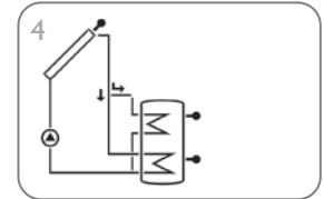
Solar system with store loading in layers (page 24)
