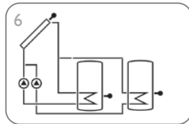
Solar system with 2 stores and pump logic (page 30)
