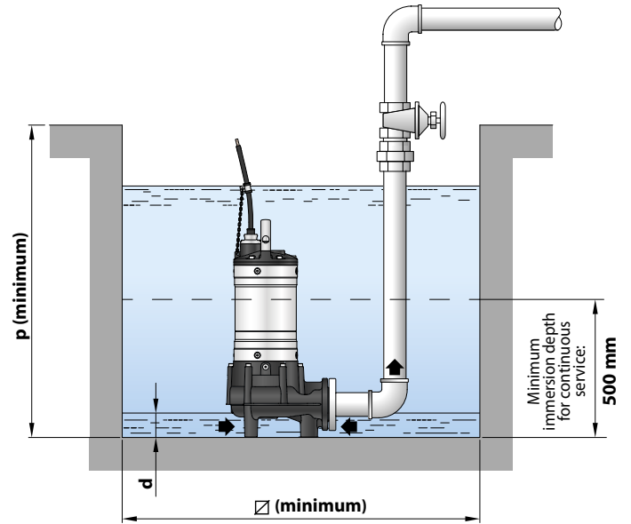
Typical installation
